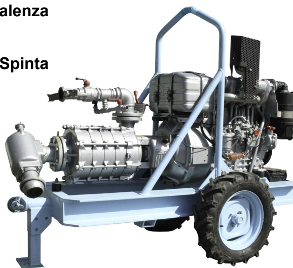
Motopompa Mod. GEO3MPCH
